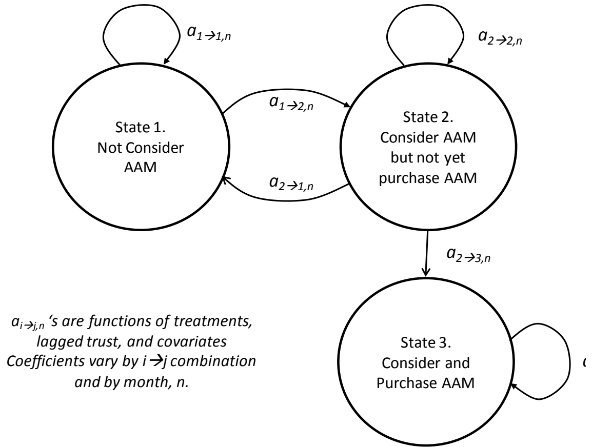
Figure A1 Continuous-Time Markov Flow Dynamics In Each Month
